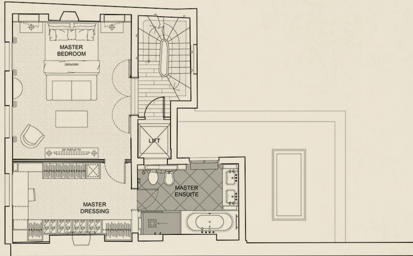
SECOND FLOOR
